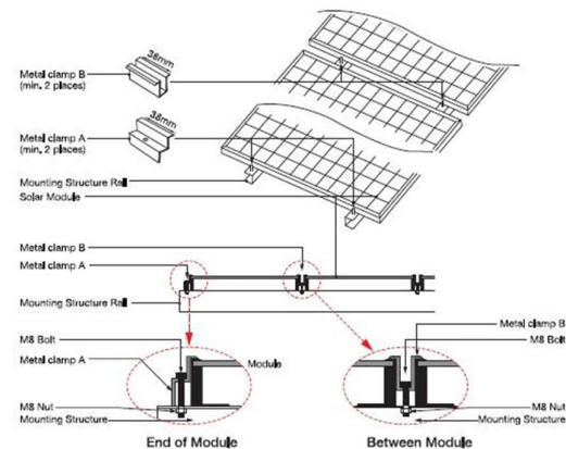
Figure 2. Mounting using clamps.
